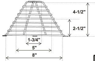
RATE OF RISE HEAT DETECTOR COVER Part No. STI 9604
