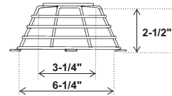
RATE OF RISE HEAT DETECTOR COVER Part No. STI 9604
