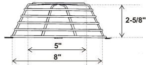
HIGH PROFILE DETECTOR COVER Part No. STI 9609
